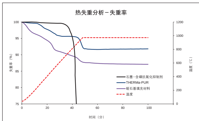
THERMa-PUR™和石墨的热失重对比试验
